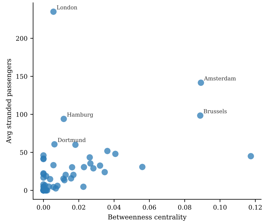
Scenario A: Northern Storm Betweenness vs stranding ( r = 0.418 )
